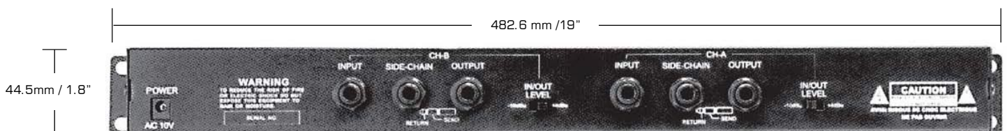
Back Panel
